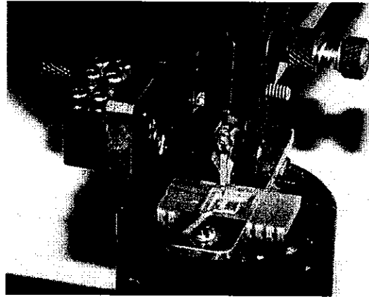
Figure 2: The depackaged smartcard processor is glued into a test package, whose pins are then connected to the contact pads of the chip with fine aluminium wires in a manual bonding machine.
